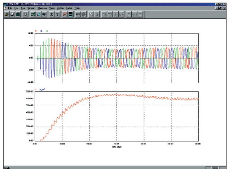
Input voltage and current waveforms
