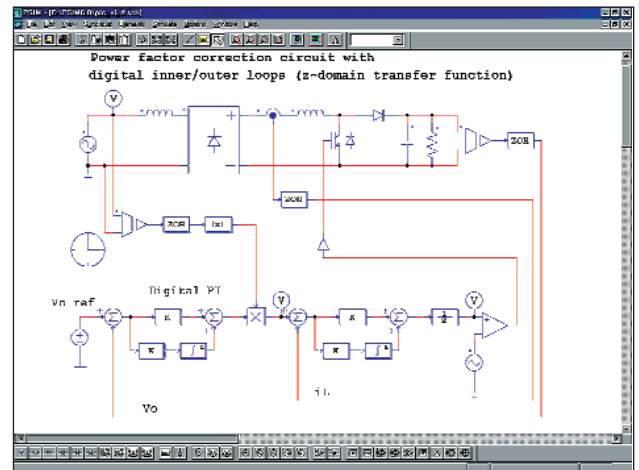
Power factor correction circuit
